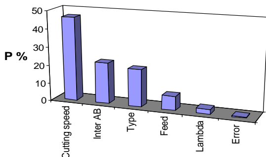
Figure 4. The influence of main factors.
