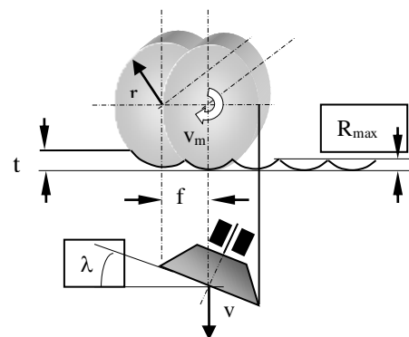
Figure 2. Peak-to-valley profile of the machined surface
