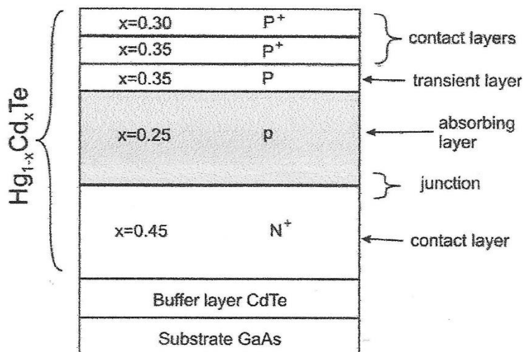
Figure 2. Example of the structure of HgCdTe photodiode (after [4]).
