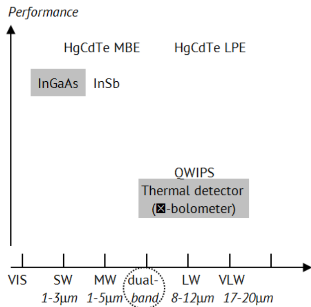
Figure 4. \text{HgCdTe} detectors grown by MBE and LPE deliver better object identification capability than the detectors, such as \otimes -bolometers and those based on InGaAs and InSb = uncooled; all other: cooled (after [7]).
