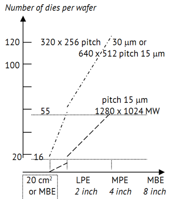
Figure 5. Switching from CdZnTe substrates to those made from Ge can substantially boots the number of dies per wafer (after [7]).
