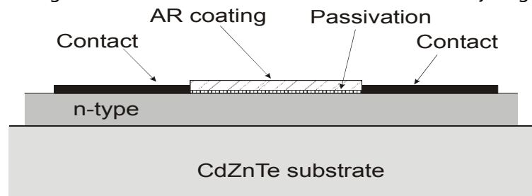
Figure 1. Cross section of a basic HgCdTe photoconductor (after [2]).
