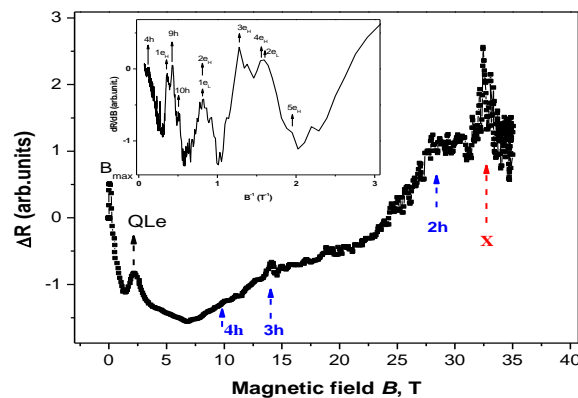
Figure 1: Longitudinal magnetoresistance for Bi wire with d = 400 nm in a magnetic field up to 35 T at T = 4.2 K. Inset: derivative dependence of resistance dR/dB as a function of 1/B in a magnetic up to 14 T.
