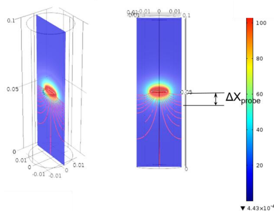
Figure 1. 2D modeling in cylindrical coordinates streamline: +Electric field Slice: Electric field norm (V/m).
