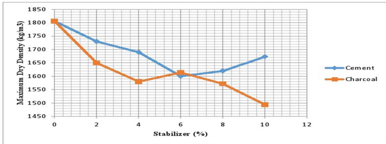
Figure 3. Variation of MDD with percentage of stabilizers.
