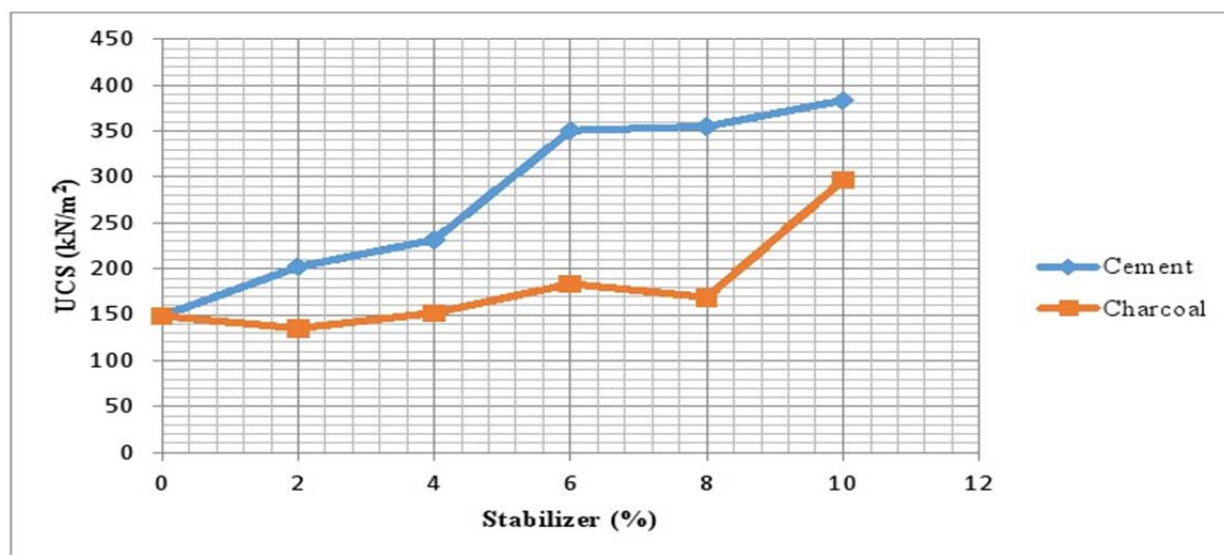
Figure 5. Variation of UCS with percentage of stabilizers.
