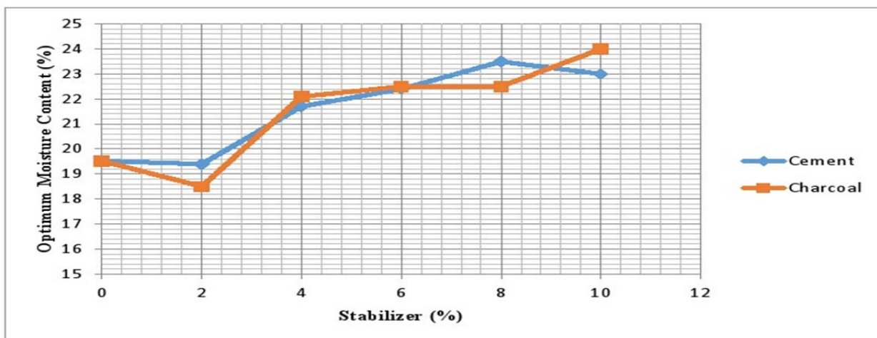
Figure 2. Variation of OMC with percentage of stabilizers.
