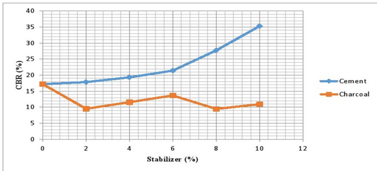
Figure 4. Variation of CBR with percentage of stabilizers.
