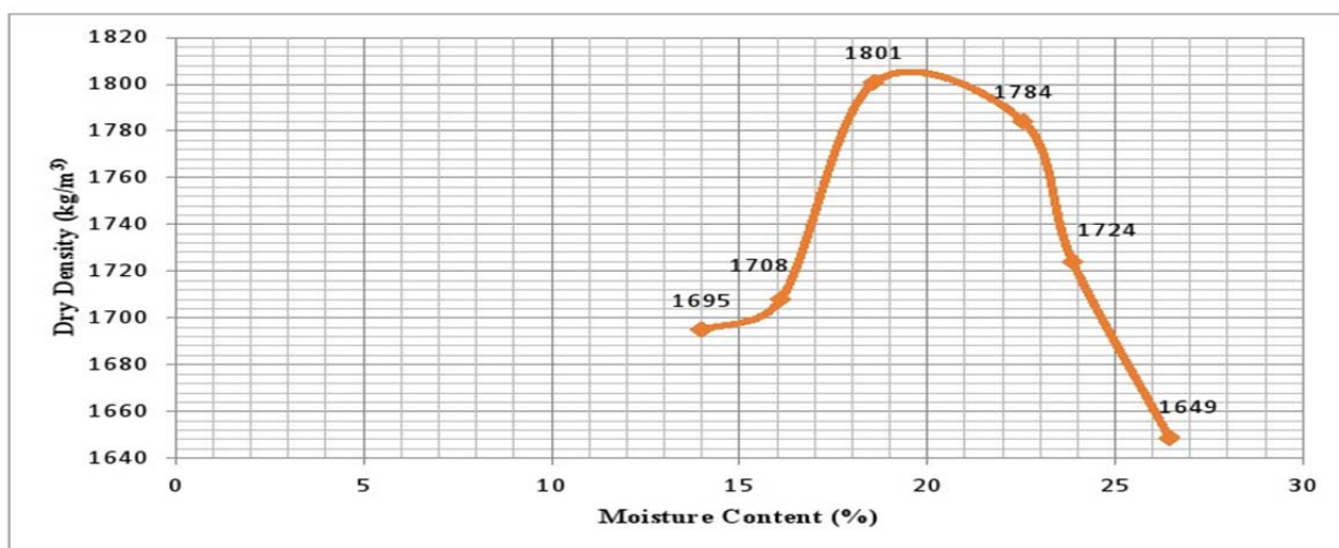
Figure 1. Compaction curve of the lateritic soil in its natural form.
