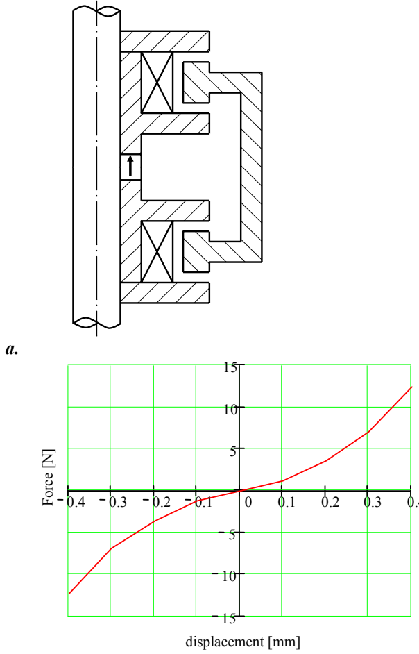
b. Figure 2. The position sensor geometry and the produced disturbing force.
